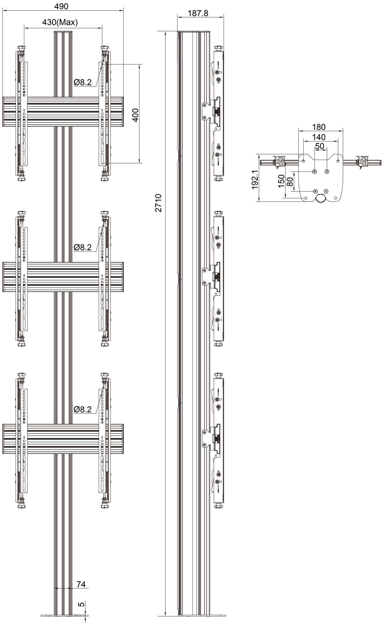
Technical measurements(mm)
