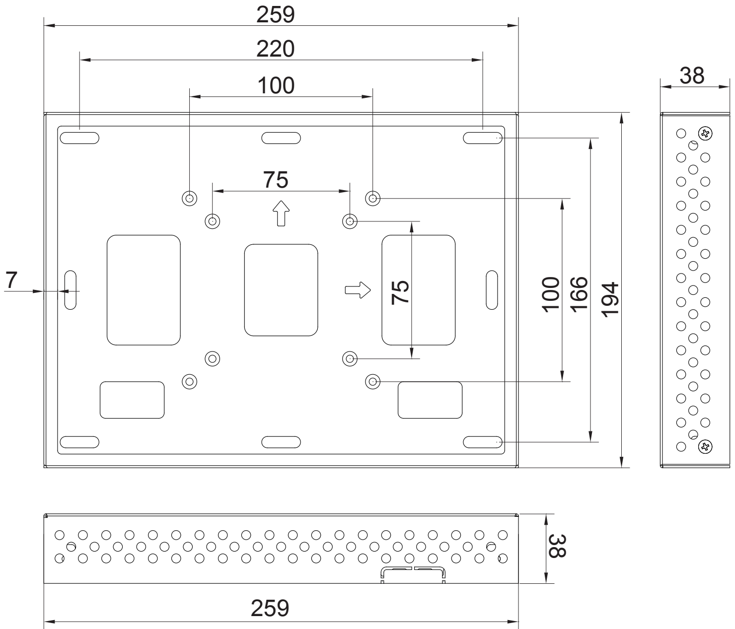
Technical measurements(mm)
