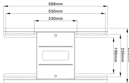
Wall plate
