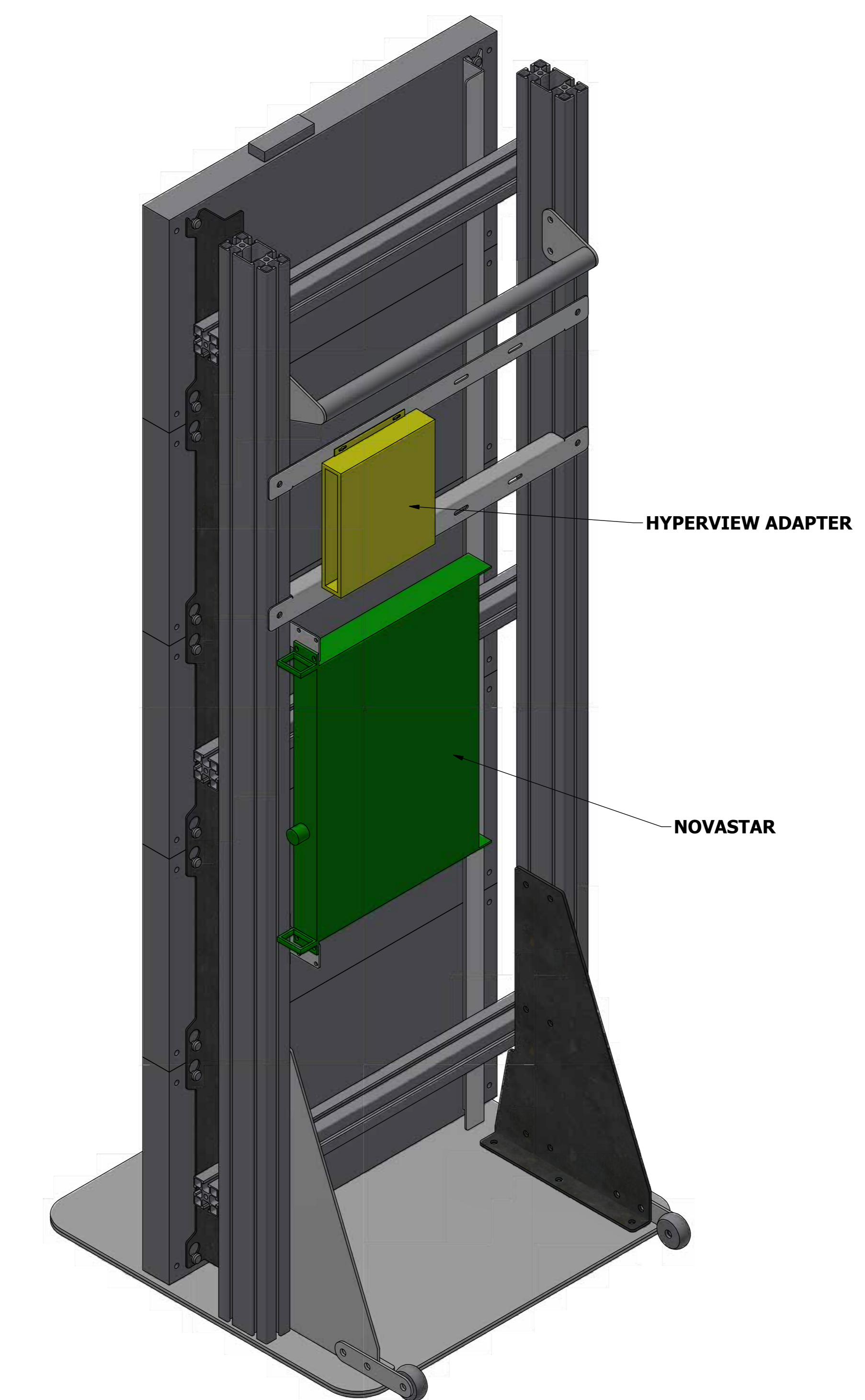
BACK VIEW WITHOUT COVER
