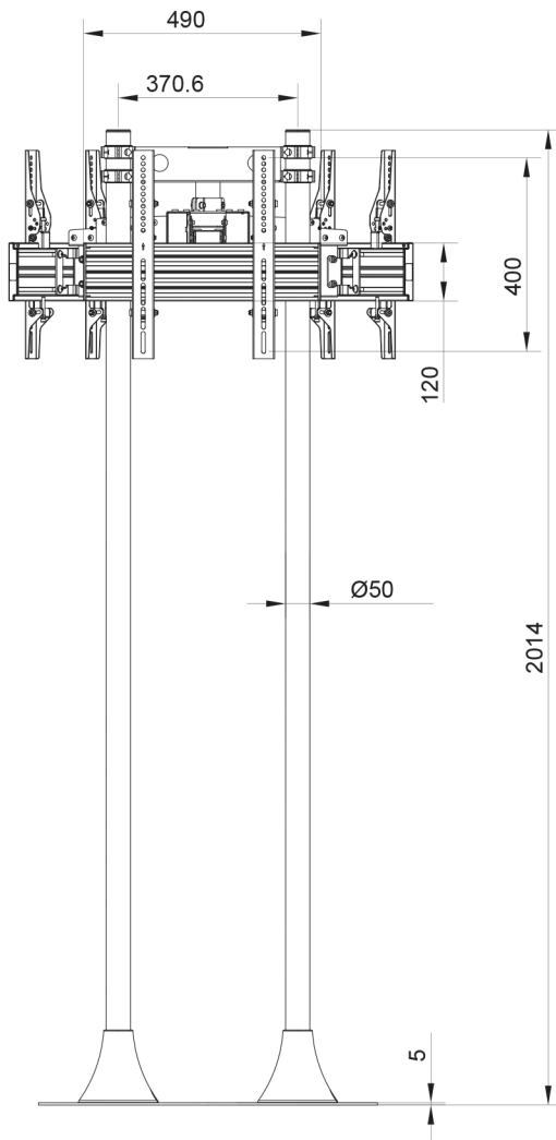
Technical measurements(mm)
