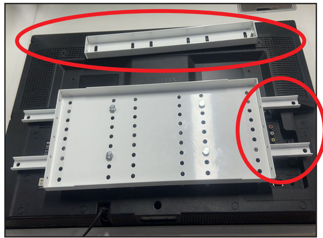
6 Fix the short VESA extension strip or lift extension plate with the long VESA Extension strips.
