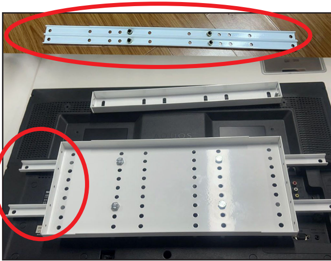
5 install the Long VESA extension strips on the back of screen.
