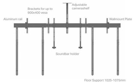
Collaboration Side by Side 90" with Floor support
