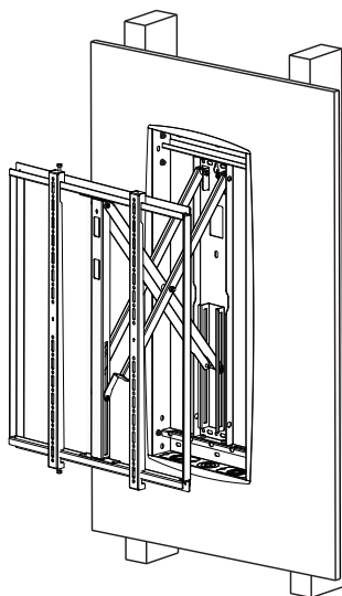
Method of installtion3
