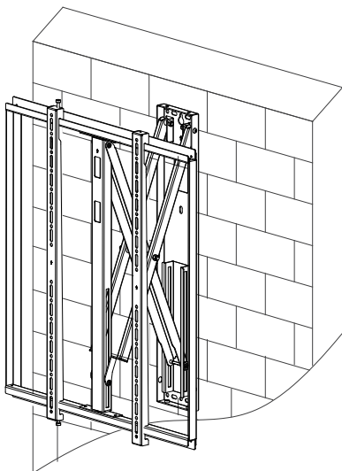
Method of installtion 2
