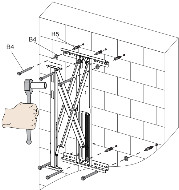
2 -B Mounting to Solid Concrete/Masonry
