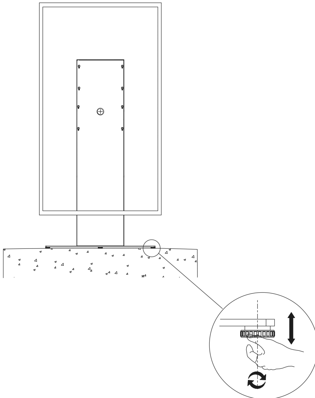
Adjustable Feet on the Bottom of Base
