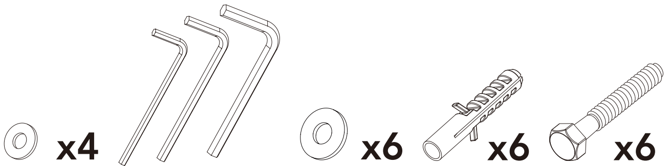
J:M5/M6 K:3/4/5mm L:M8 M:Anchor N:M8x50mm
