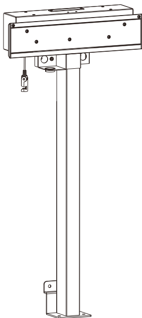
J:M5/M6 K:3/4/5mm L:M8 M:Anchor N:M8x50mm
