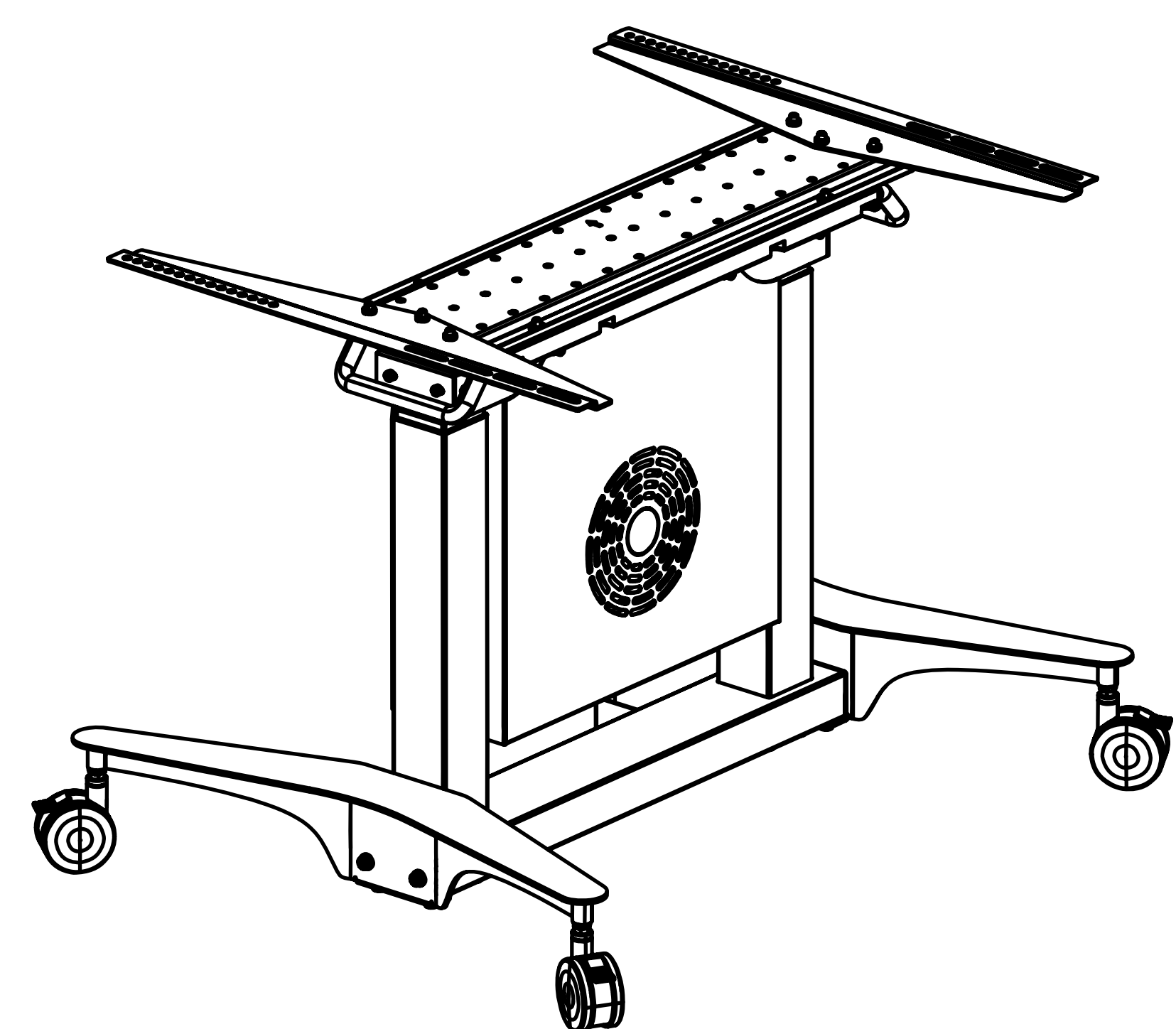
Horizontal position
