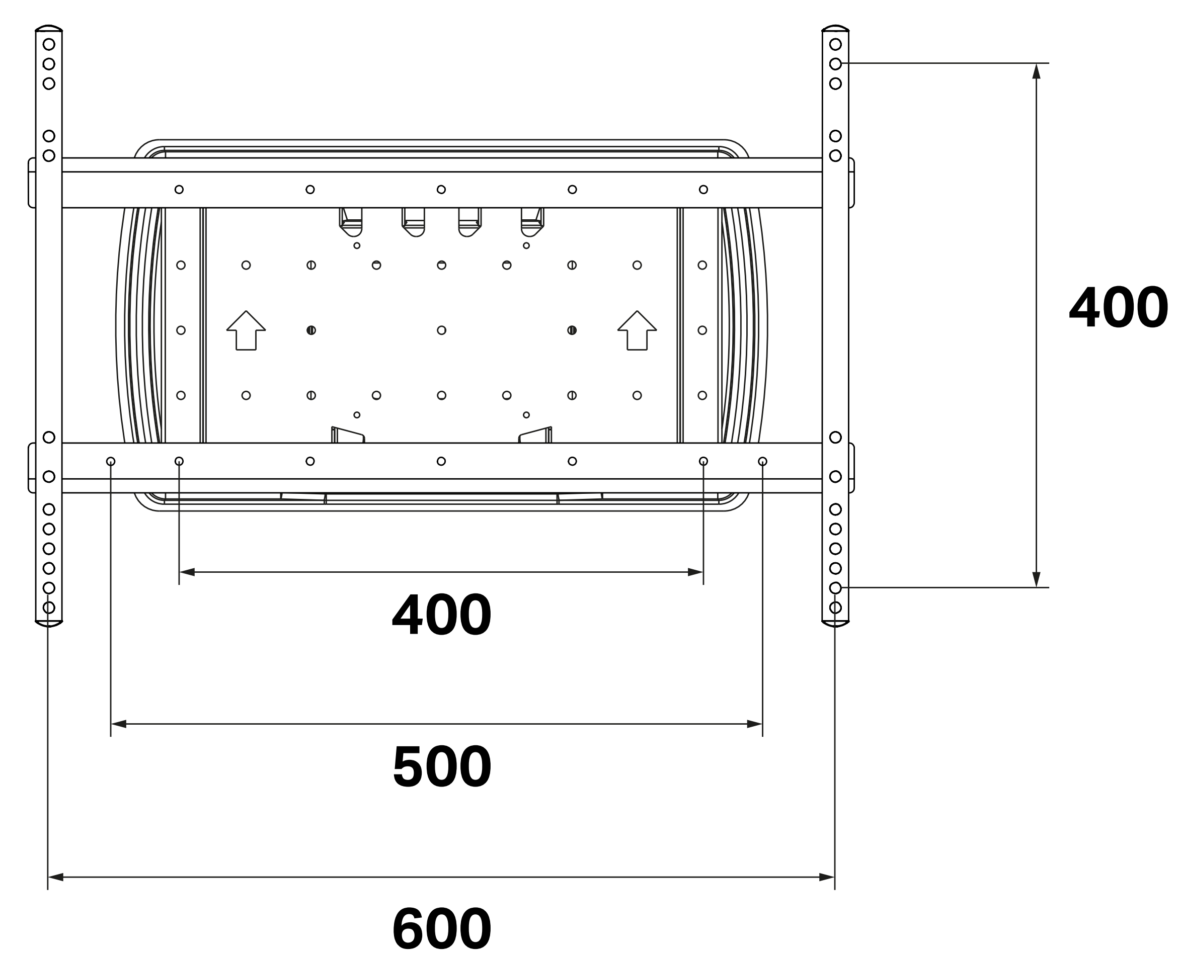
M VESA Super Slim Tilt & Turn SD EAN: 735002273 8249
