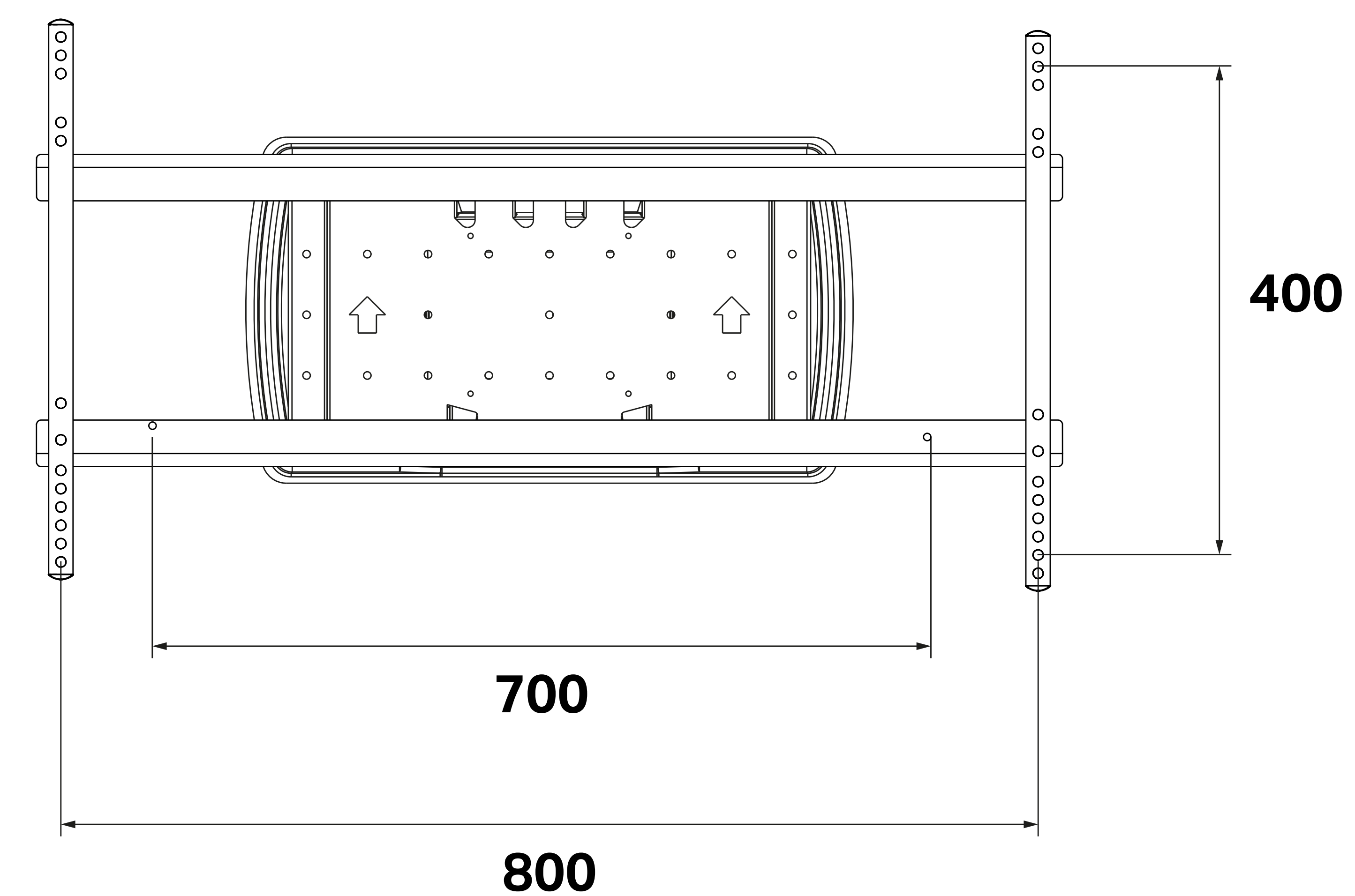
M VESA Super Slim Tilt & Turn SD 800 EAN: 735002273 9901
