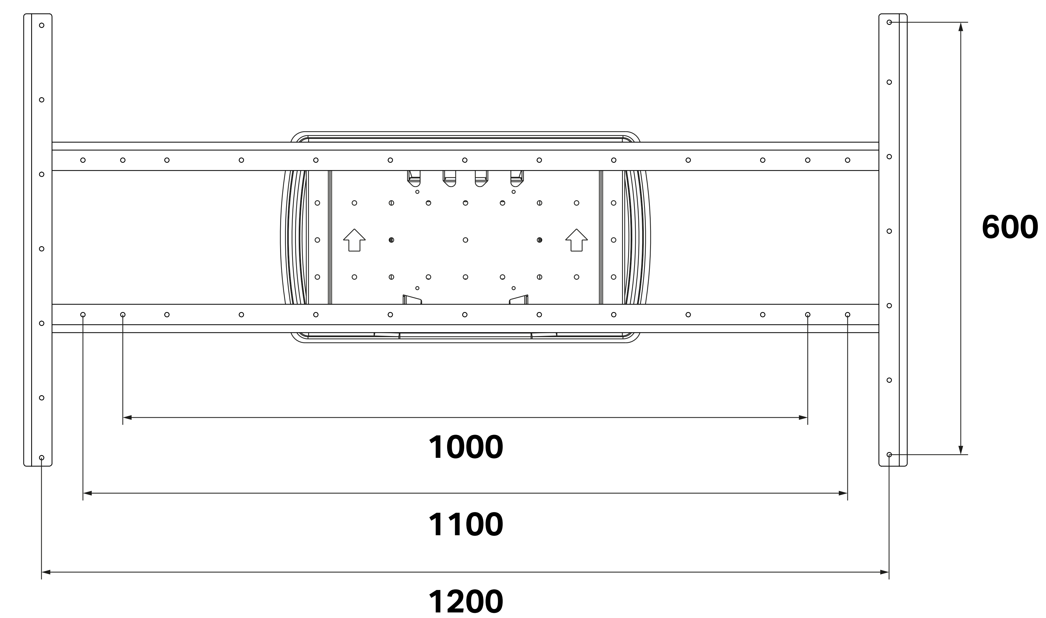
M VESA Super Slim Tilt & Turn SD 1200 EAN: 735002273 9925
