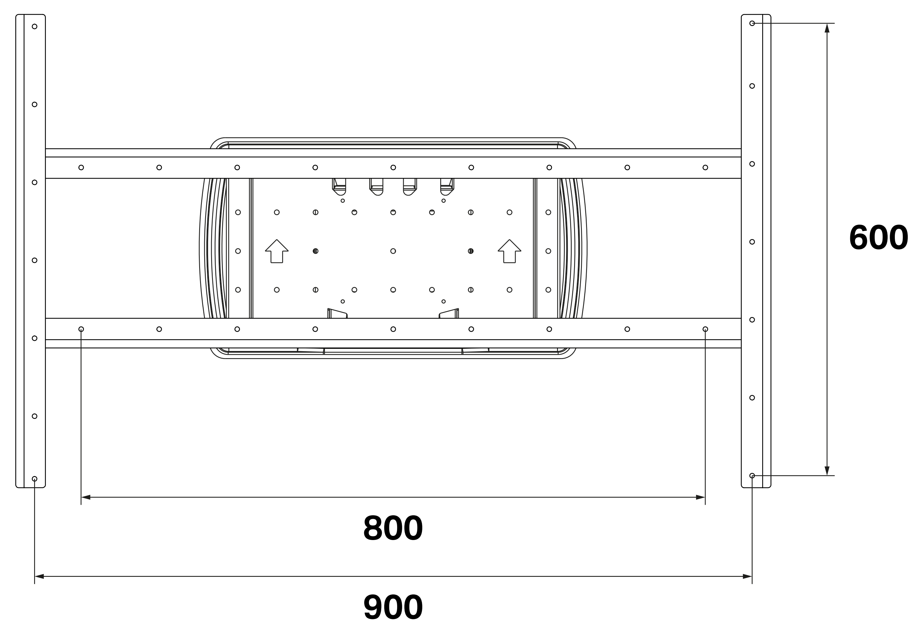
M VESA Super Slim Tilt & Turn SD 900 EAN: 735002273 9918
