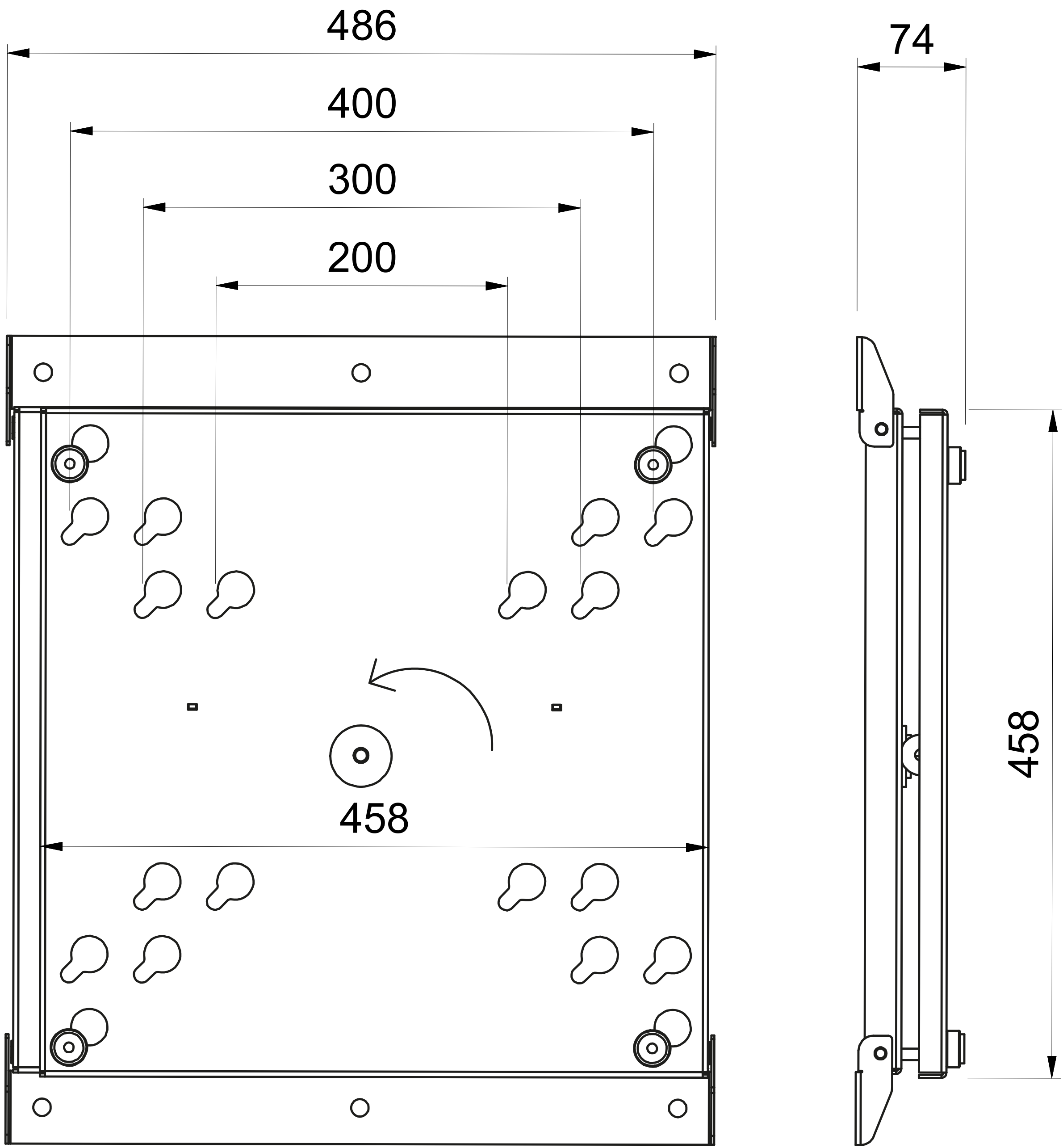
VESA 200-300-400 Landscape
