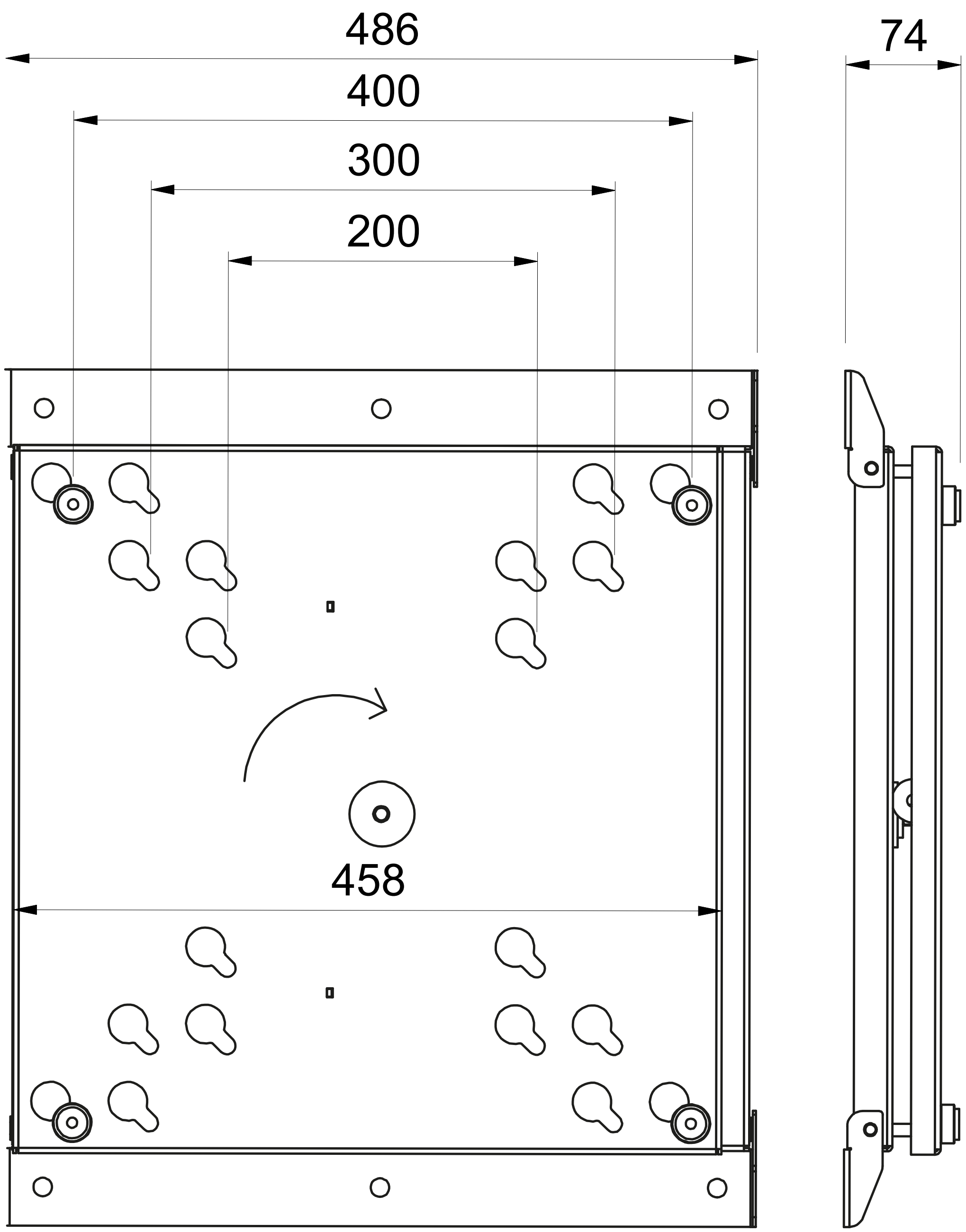
VESA 200 - 300 - 400 Portrait
